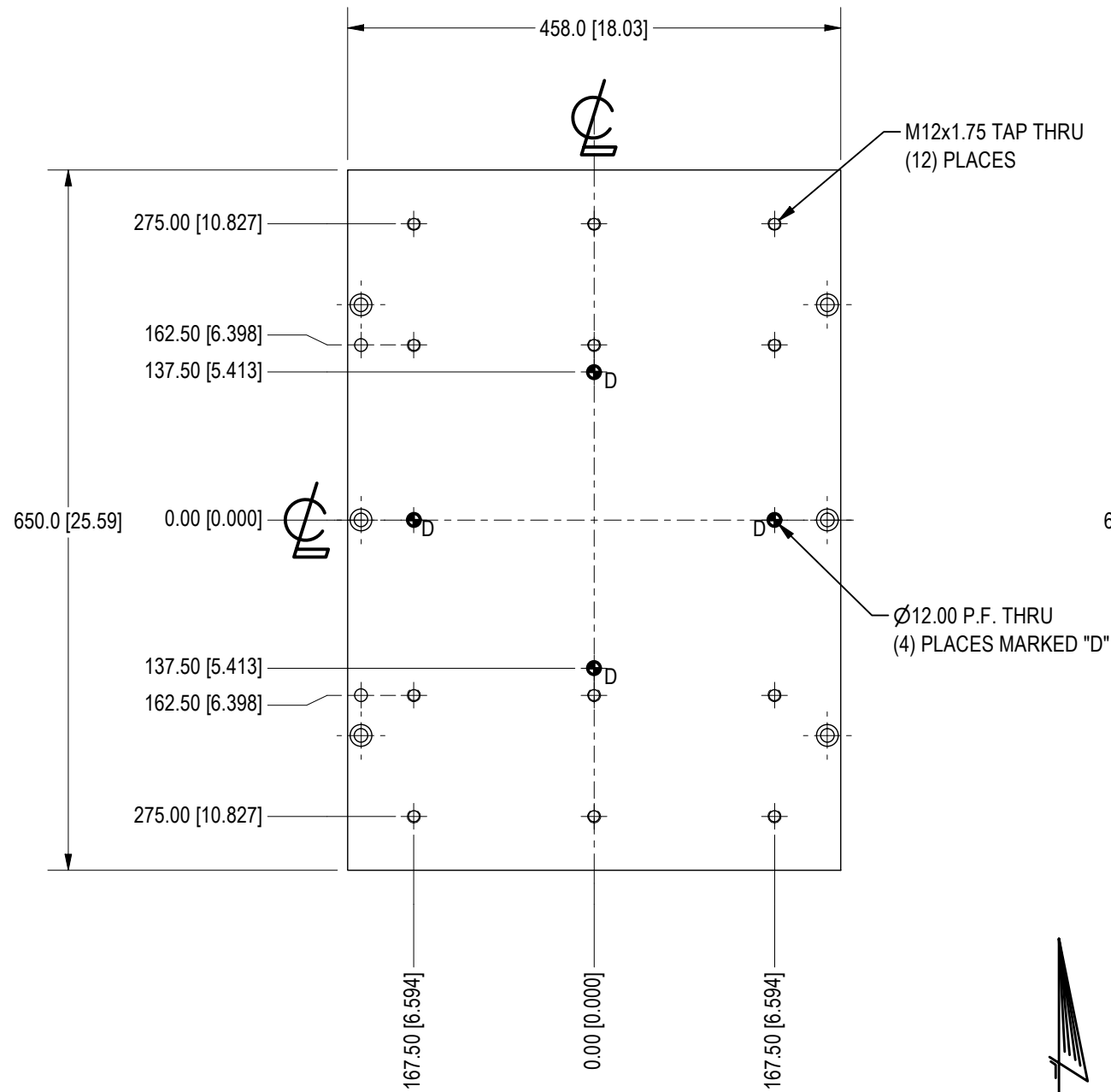
3 BEARING NARROW MOUNTING PLATE
